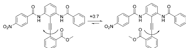
Scheme 1. A bisbenzamido-diphenylacetylene scaffold where the conformational equilibrium is biased by the differential acidity of the flanking benzamides. [4]
